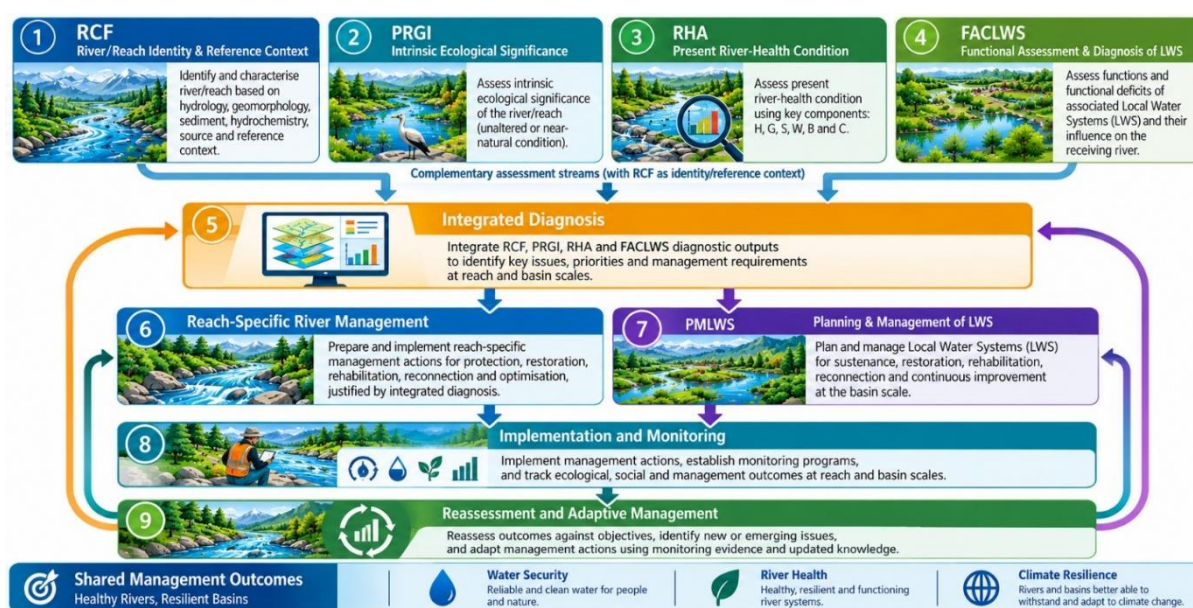
Figure 1.1: Integrated River Assessment Framework (IRAF) - From River Classification and Integrated Diagnosis to Planning, Management and Outcomes
