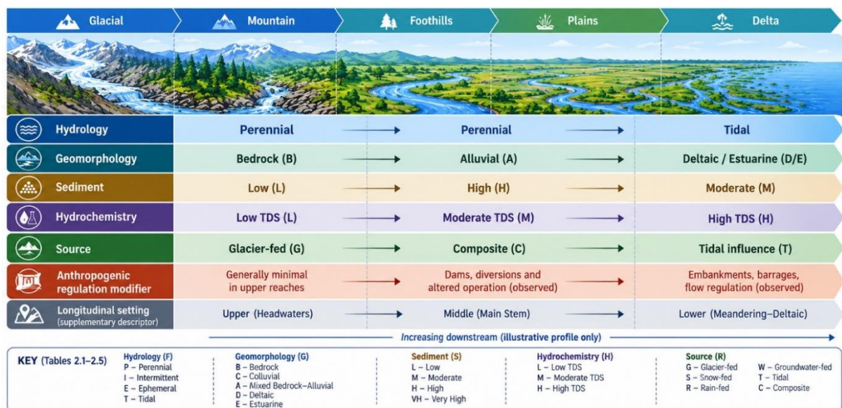
Figure 7.1: Typical Longitudinal Profile of a River
