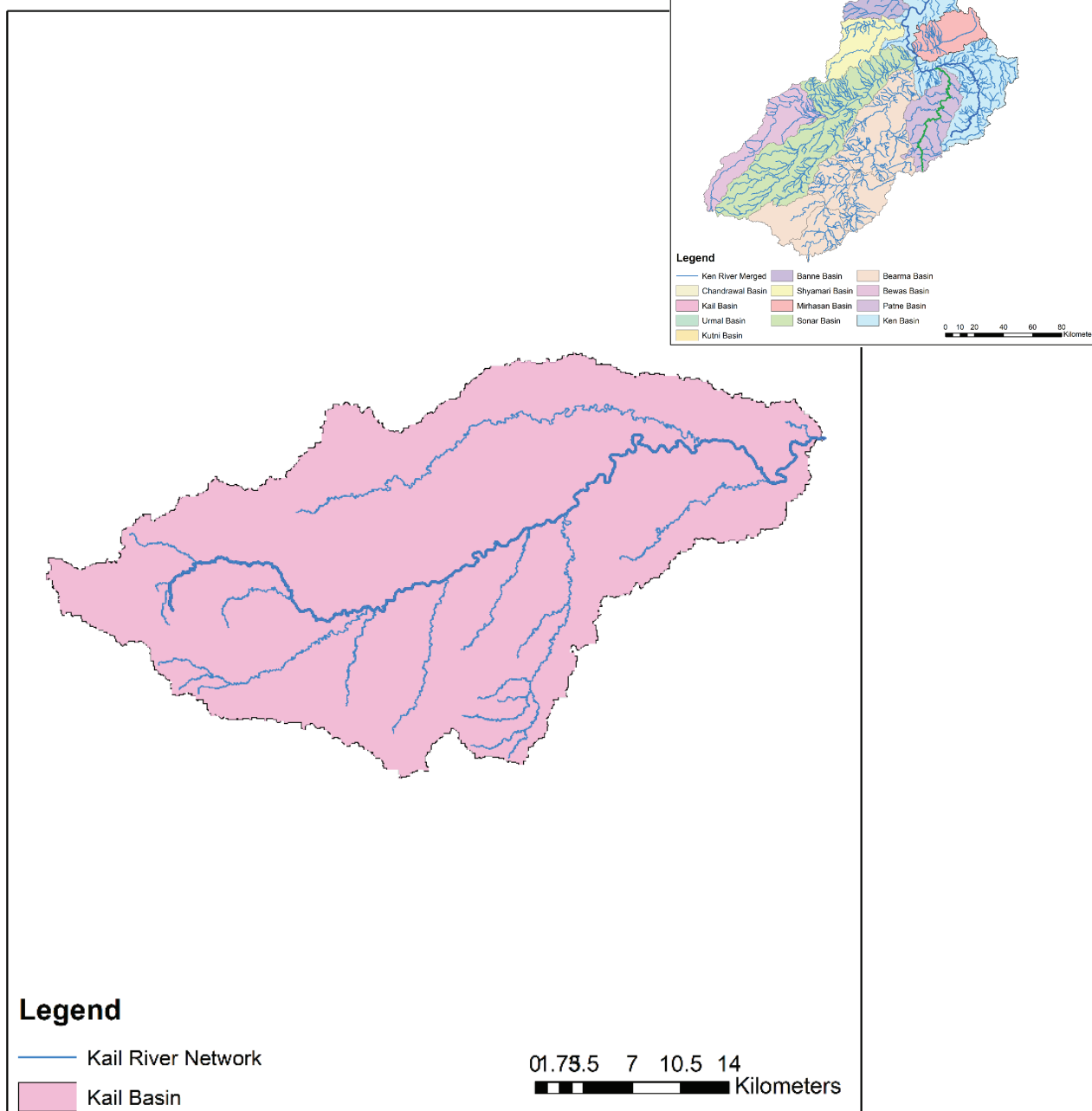
Figure: Kail River Network
