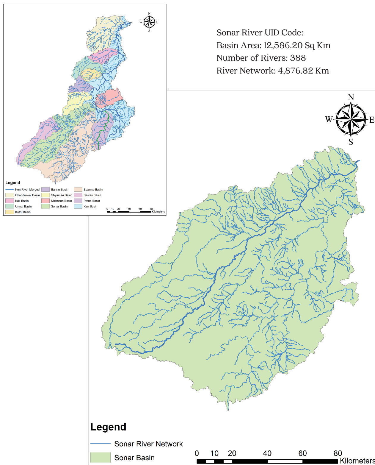
Figure: Sonar River Network
