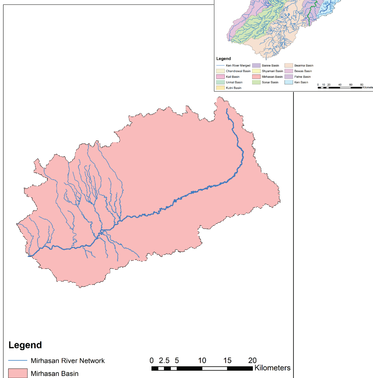
Figure: Mirhasan River Network
