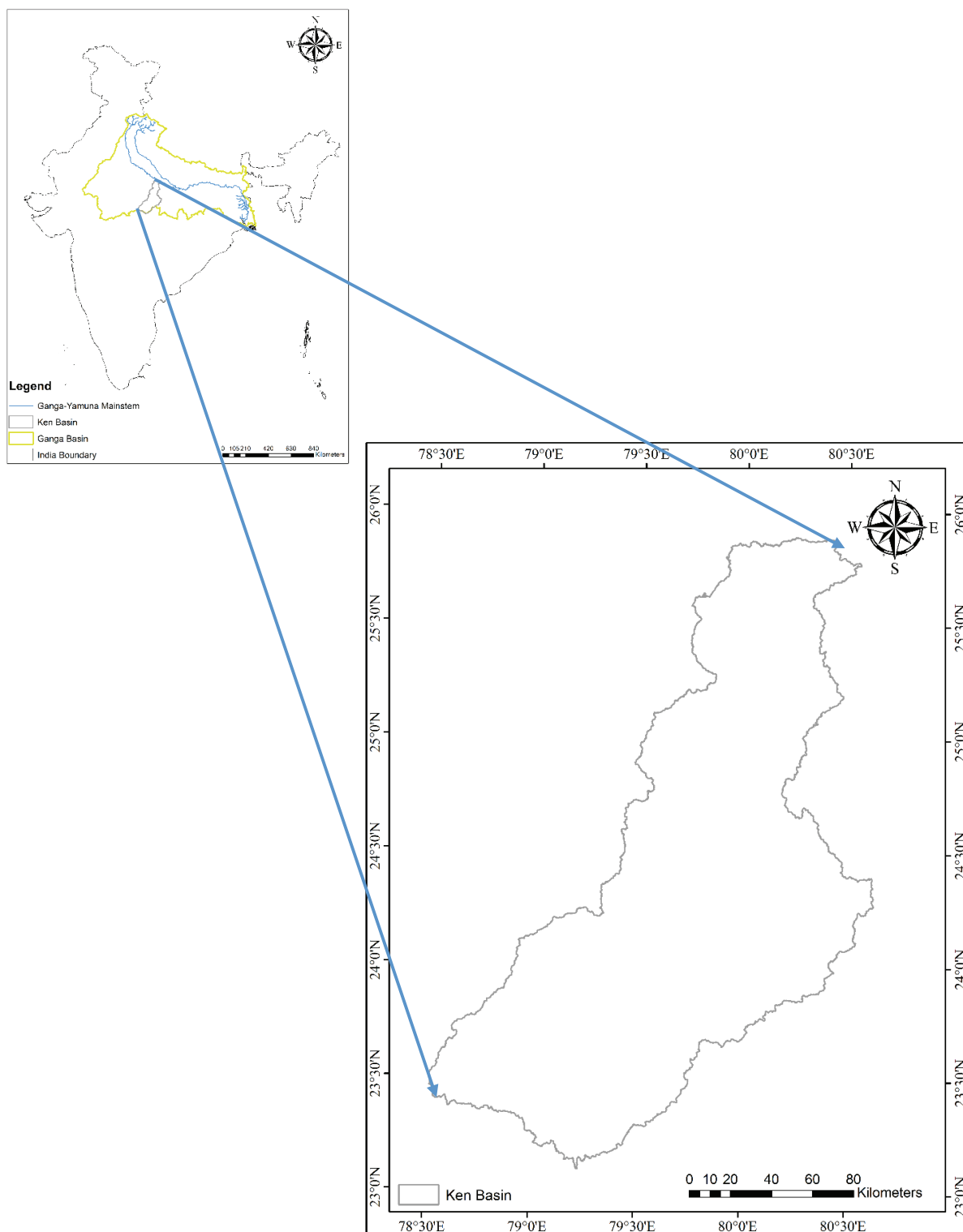
Figure: Location of Ken Basin
