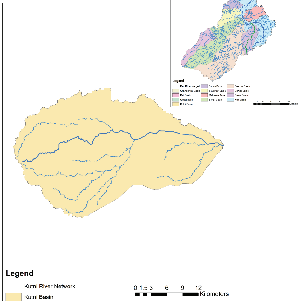
Figure: Kutni River Network
