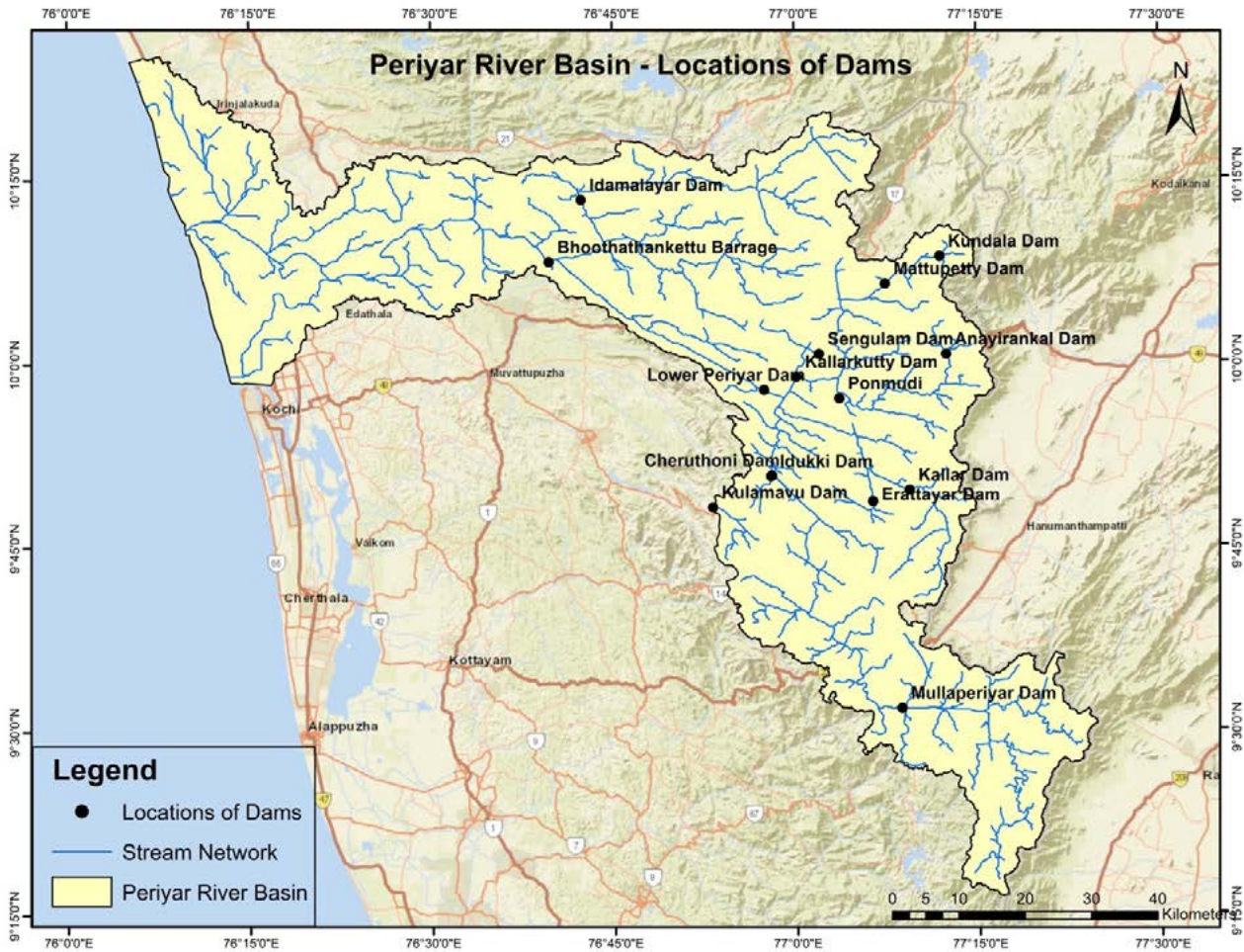
Fig. 3 Location of Major dams in the basin
