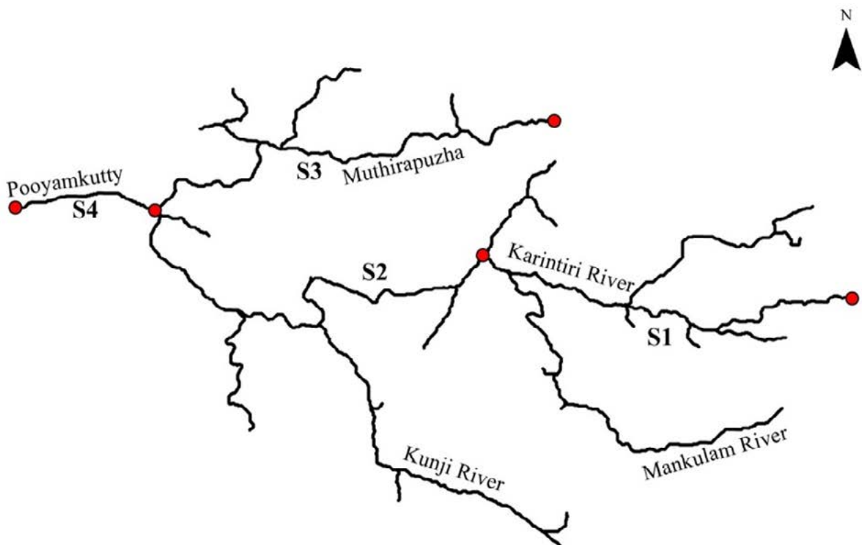
Fig. 10 e River Segmentation for Pooyamkutty
