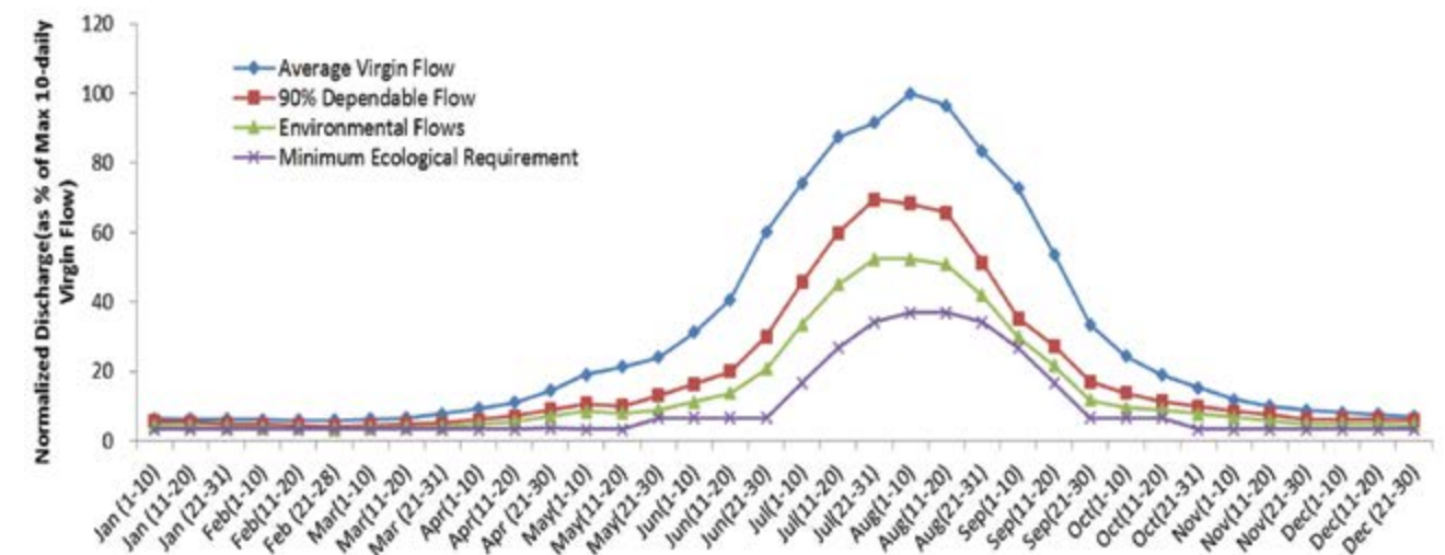
Figure 8: Computed 10-daily E-Flows at Ranari, Dharasu
